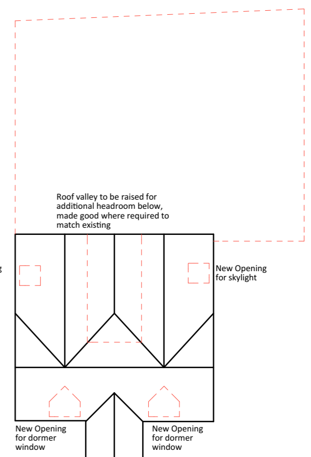
Roof Floor
